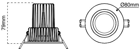
CUT-OUT: Ø70mm
