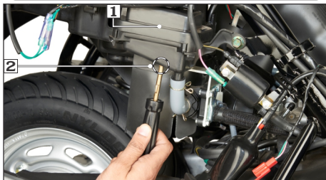
(1) Air cleaner element housing cover (2) Screw
