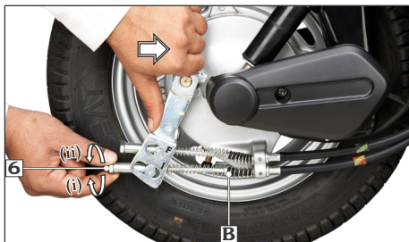
(6) Second adjuster nut (i) Decrease free play (ii) Increase free play
