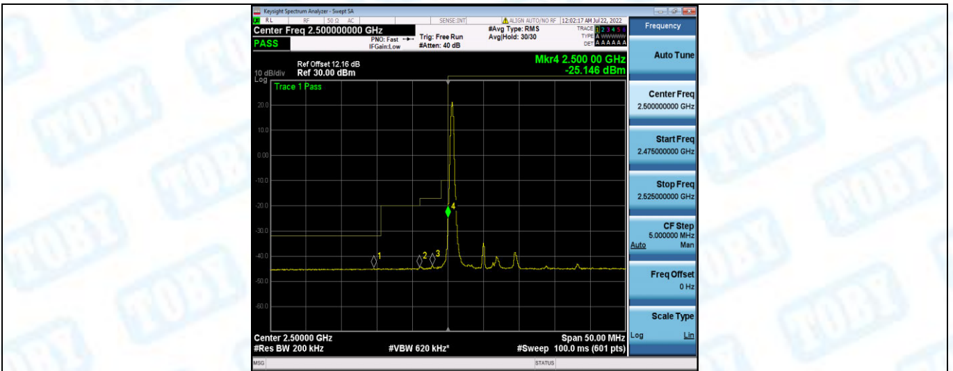
Band7-10MHz-QPSK-20800-1RB#49
