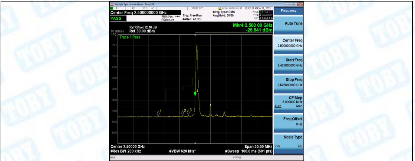
Band7-10MHz-16QAM-20800-1RB#49
