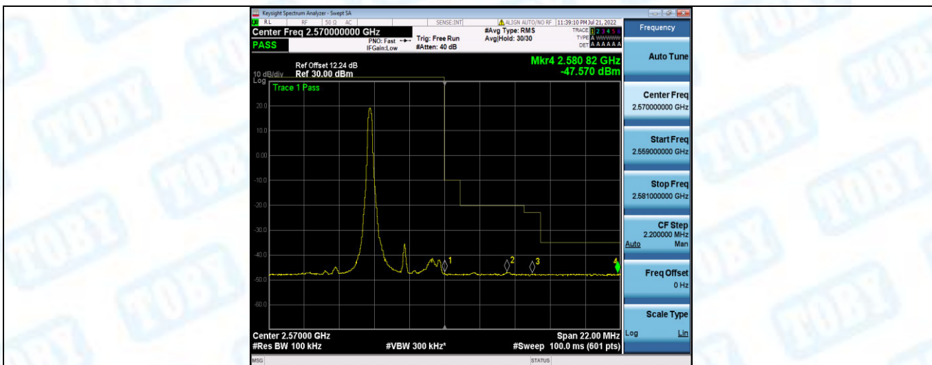
Band7-5MHz-QPSK-21425-1RB#24
