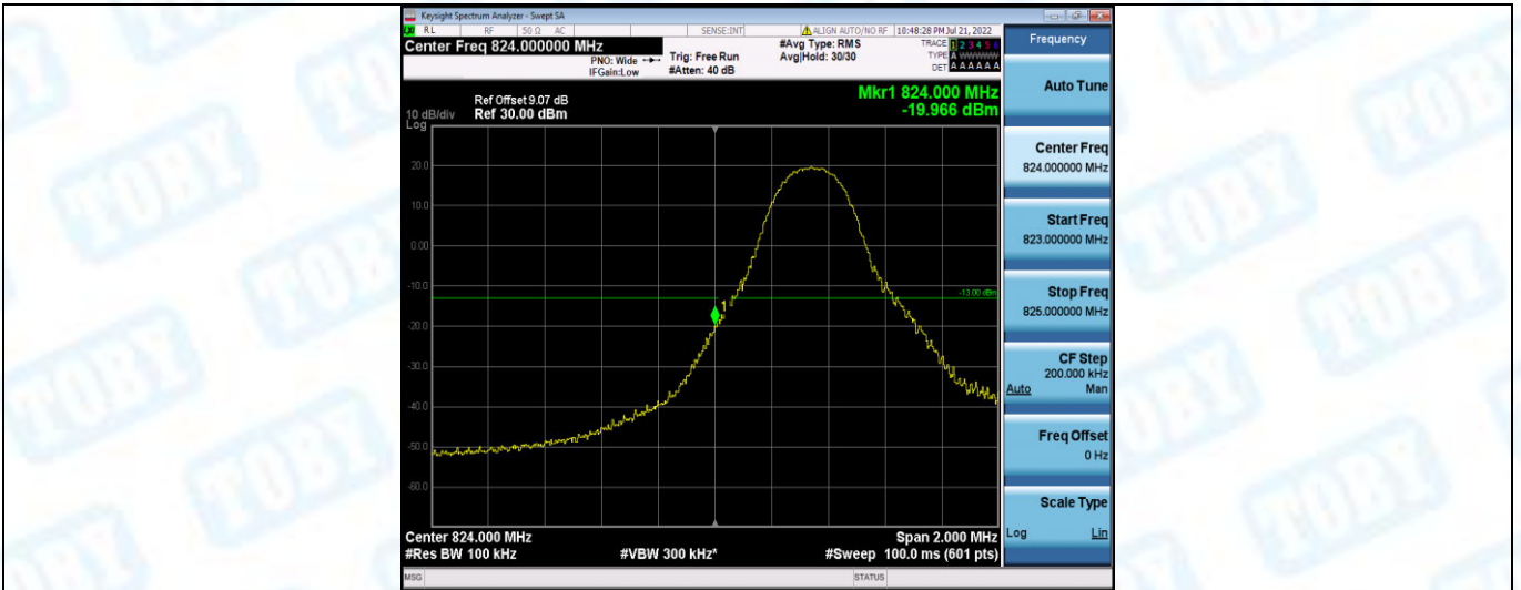
Band5-5MHz-16QAM-20425-1RB#24
