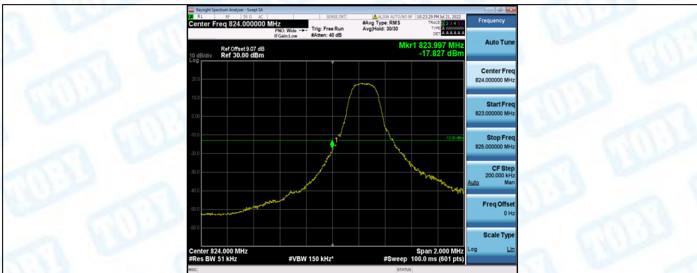
Band5-3MHz-QPSK-20415-1RB#14
