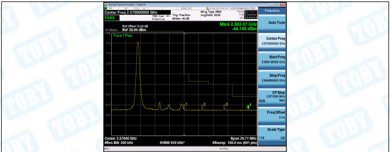
Band7-10MHz-QPSK-21400-1RB#49
