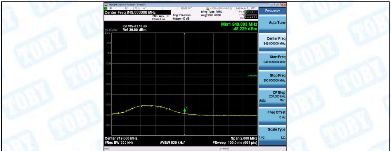
Band5-10MHz-QPSK-20600-1RB#49
