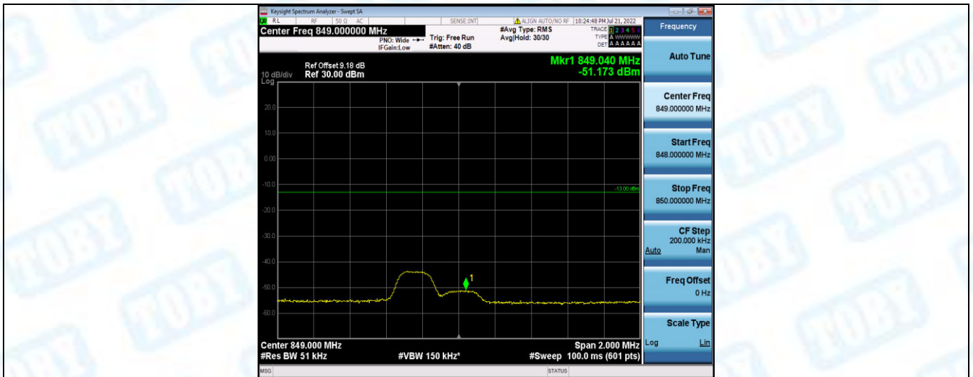
Band5-3MHz-16QAM-20635-1RB#14
