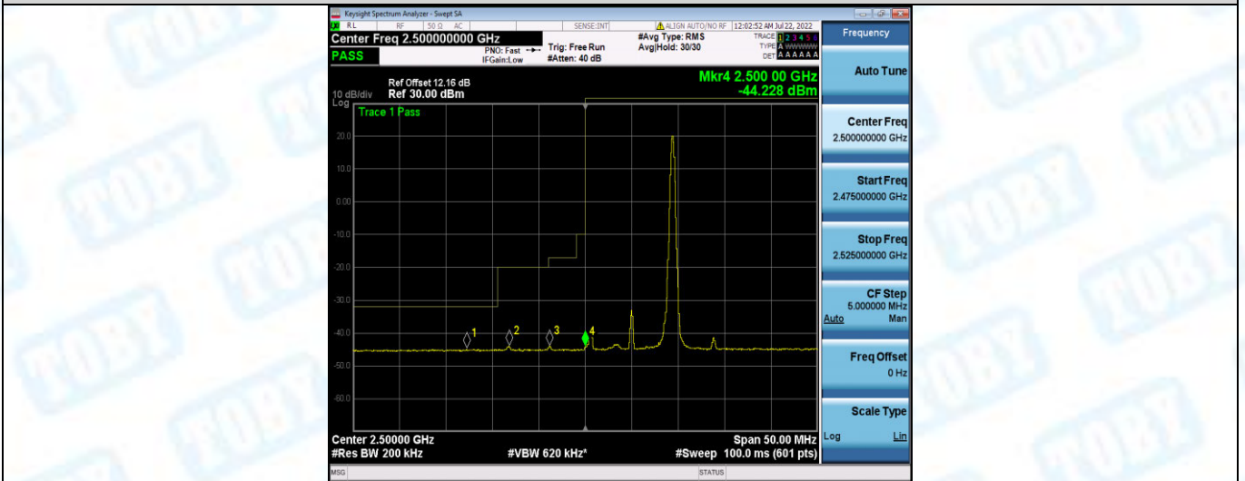
Band7-10MHz-16QAM-20800-50RB#0
