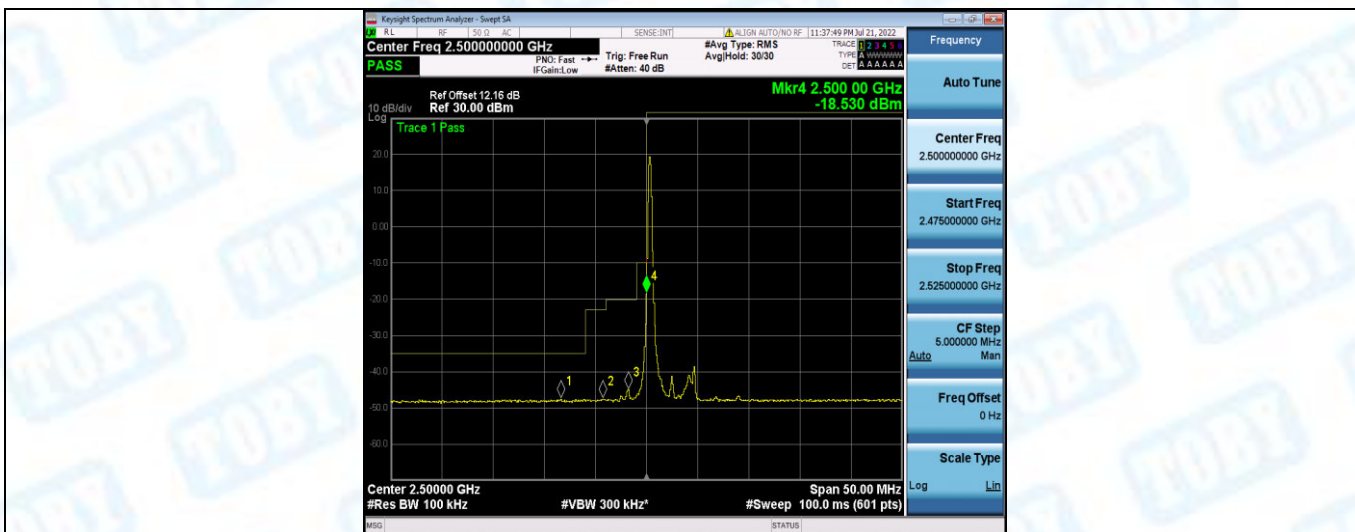
Band7-5MHz-QPSK-20775-1RB#24
