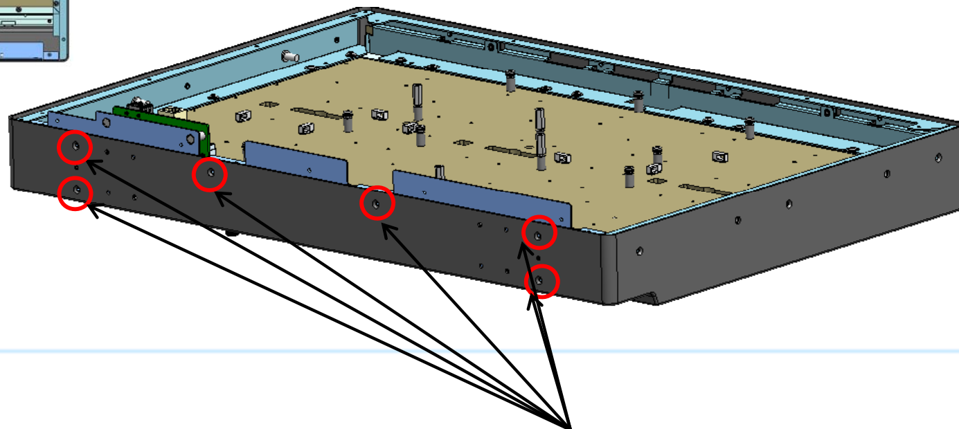
SCREW-Ax6
