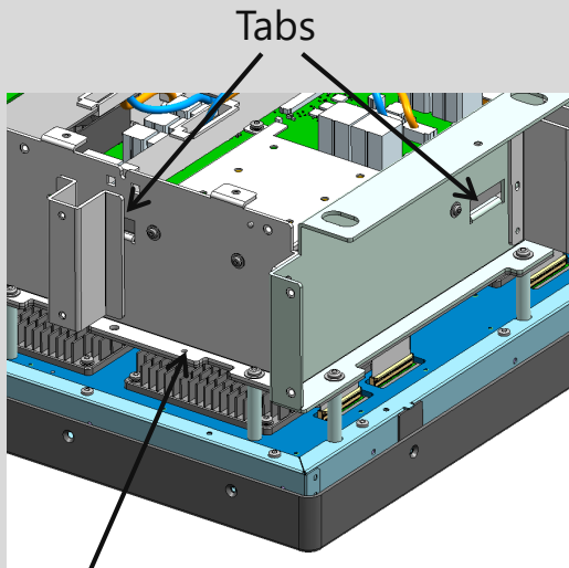
Positioning mark
