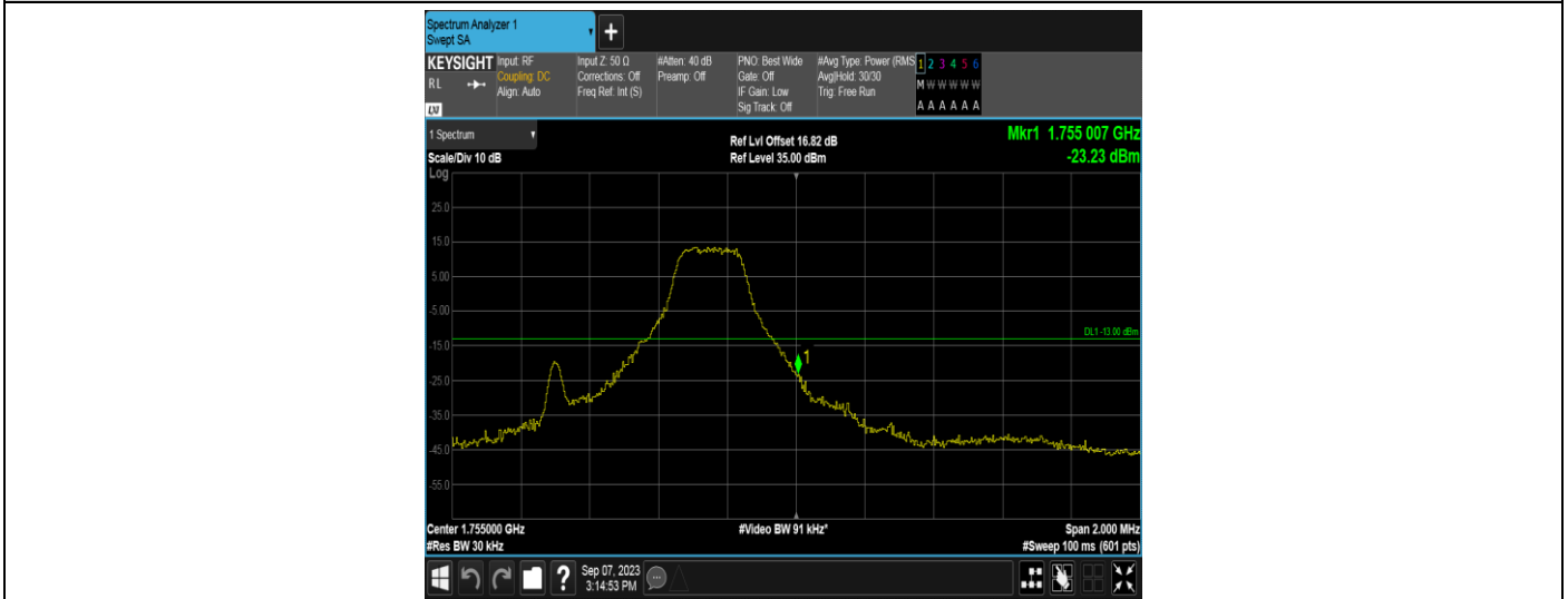
Band4-1.4MHz-QPSK-20393-1RB#5
