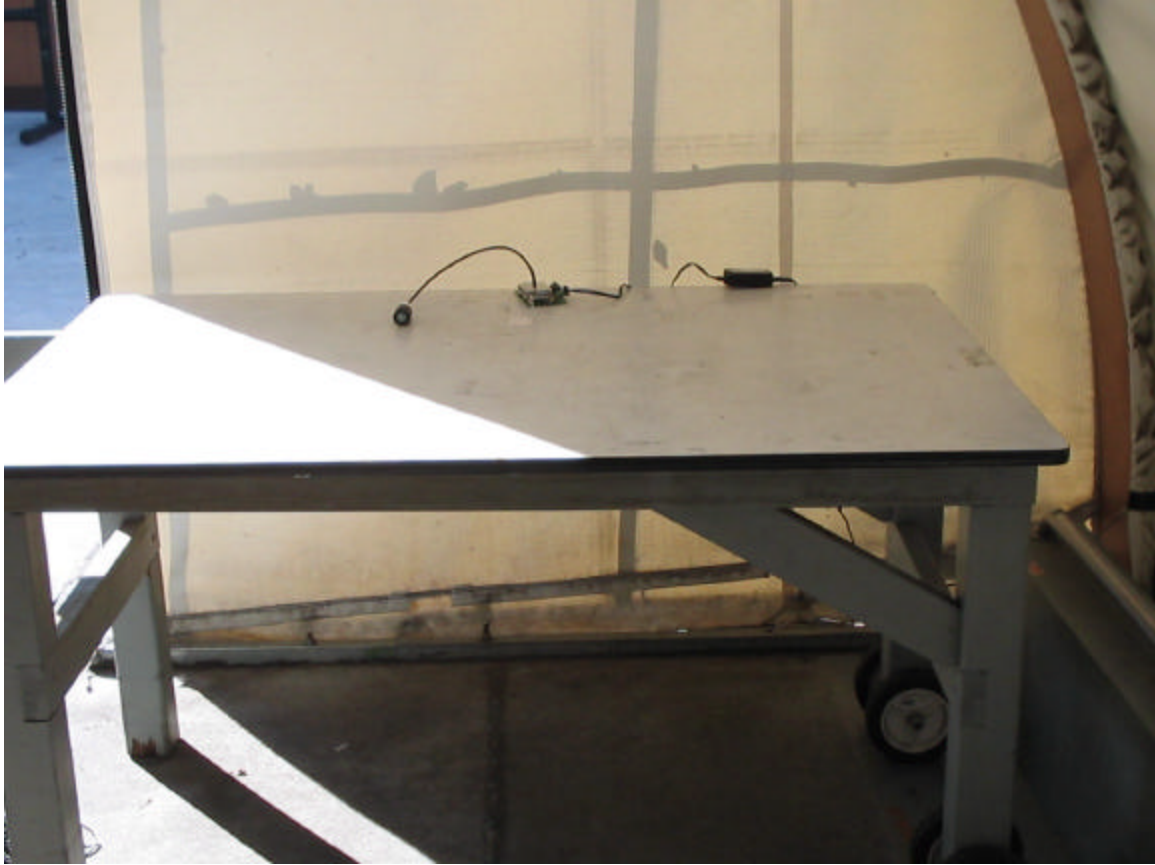
AC CONDUCTED EMISSION SETUP PHOTO
