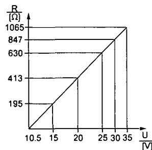
FMX21 load chart for estimating the load resistance. Additional resistances, such as the resistance of the extension cable, have to be subtracted from the value calculated as shown in the equation.
