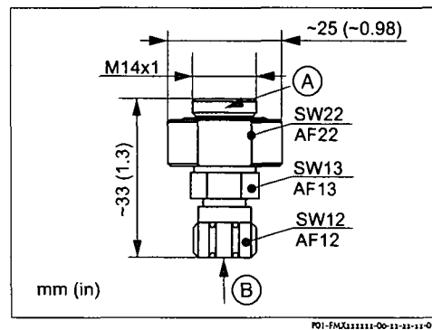
Testing adapter
