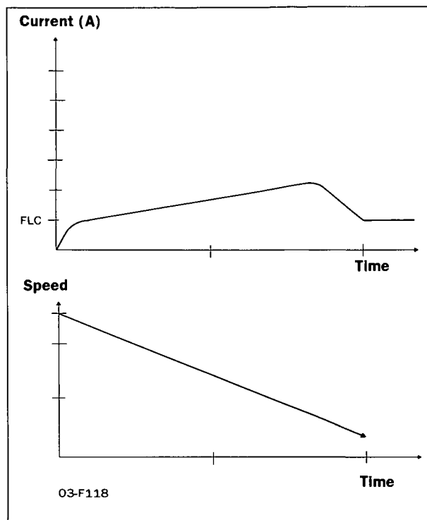
Fig. 36 Pump control
