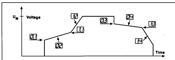
Fig. 33 Menu numbers for dual voltage ramp at start/stop, initial voltage at start and step down-voltage at stop.
