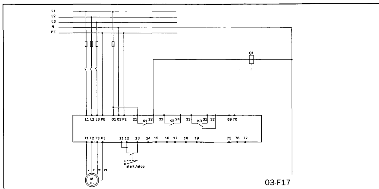
Fig. 6 Standard wiring.
