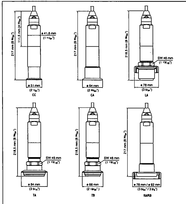
Fig. 12: VEGABAR 74 - hygienic fitting: CC = Tri-Clamp 1½", CA = Tri-Clamp 2", LA = hygienic fitting with compression nut F40, TA = Tuohenhagen Varivent DN 32, TB =
