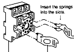
Socket SR2P-05 Hold-down Spring (sold separately) SFA-203 (use two springs)
