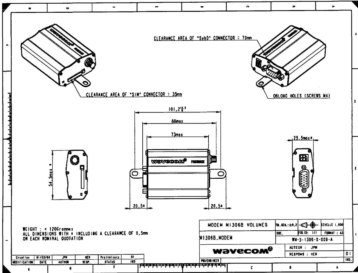
Figure 18: Dimensioning diagram
