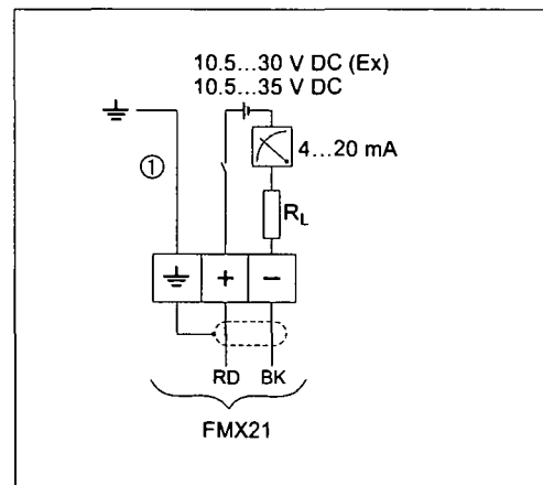
Electrical connection
