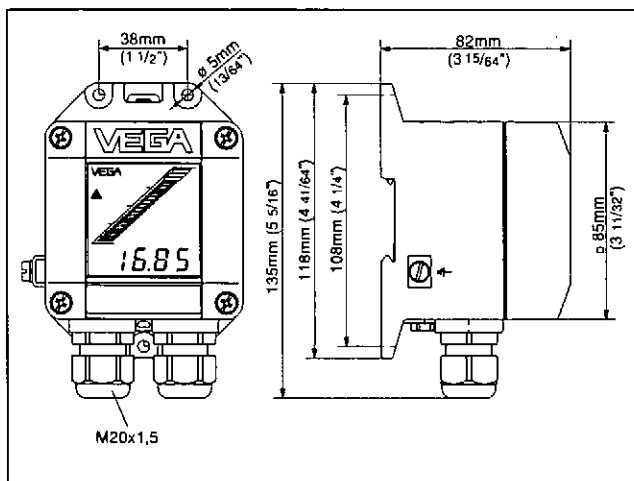
Fig. 26: VEGADIS 11, 12
