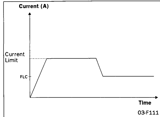
Fig. 4 Current control
