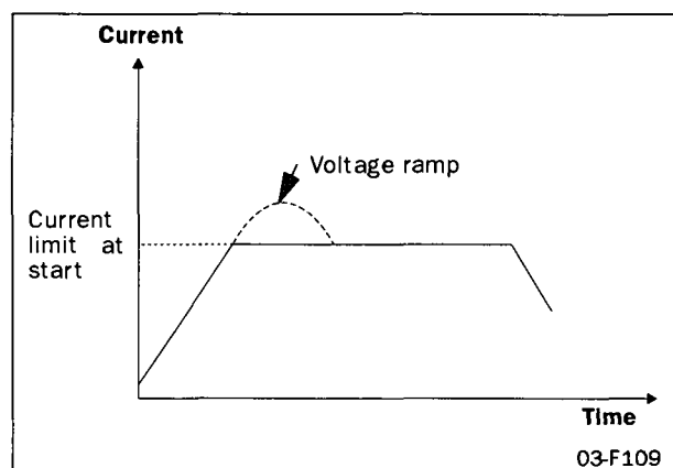
Fig. 34 Current limit
