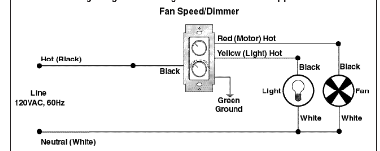
Wiring Diagram 1 - Single Location Control Application
