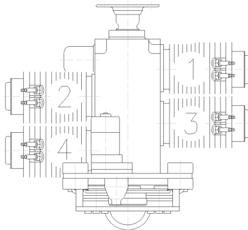
Figure 3 – 2200 Cylinder Denomination
