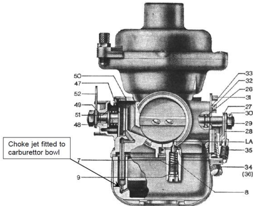
Figure 49 – Choke Schematic
