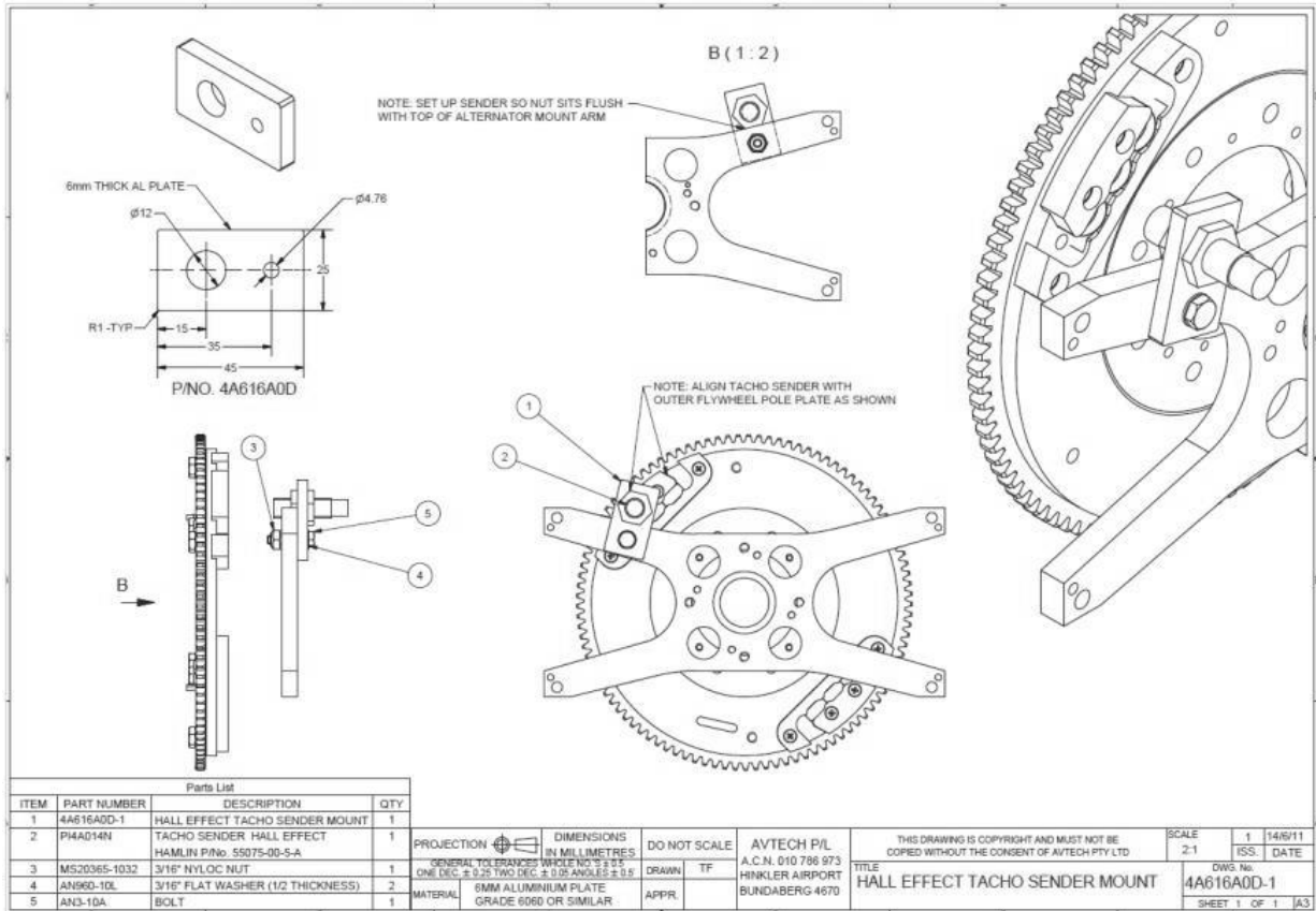
Figure 38 – Tacho Sender #2
