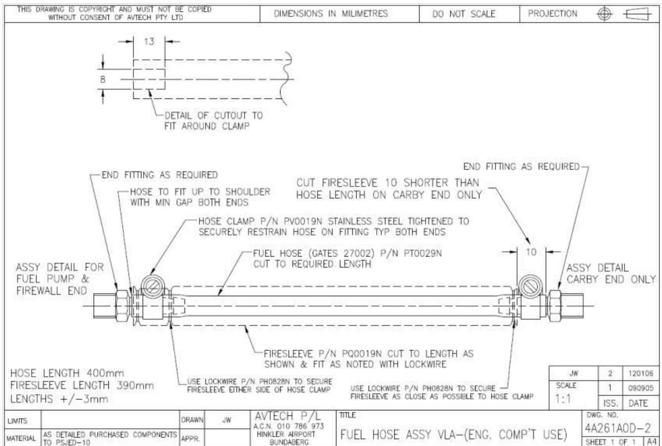
Figure 36 – Fuel Hose Assembly – Engine Bay
