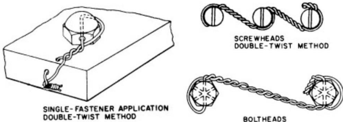
Figure 46 – Safety Wire Details
