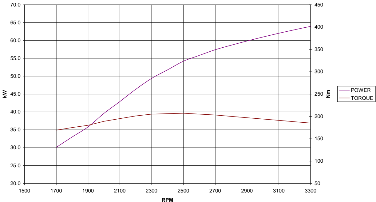
Figure 7 – Power / Torque Curve – Typical 2200A Engine
