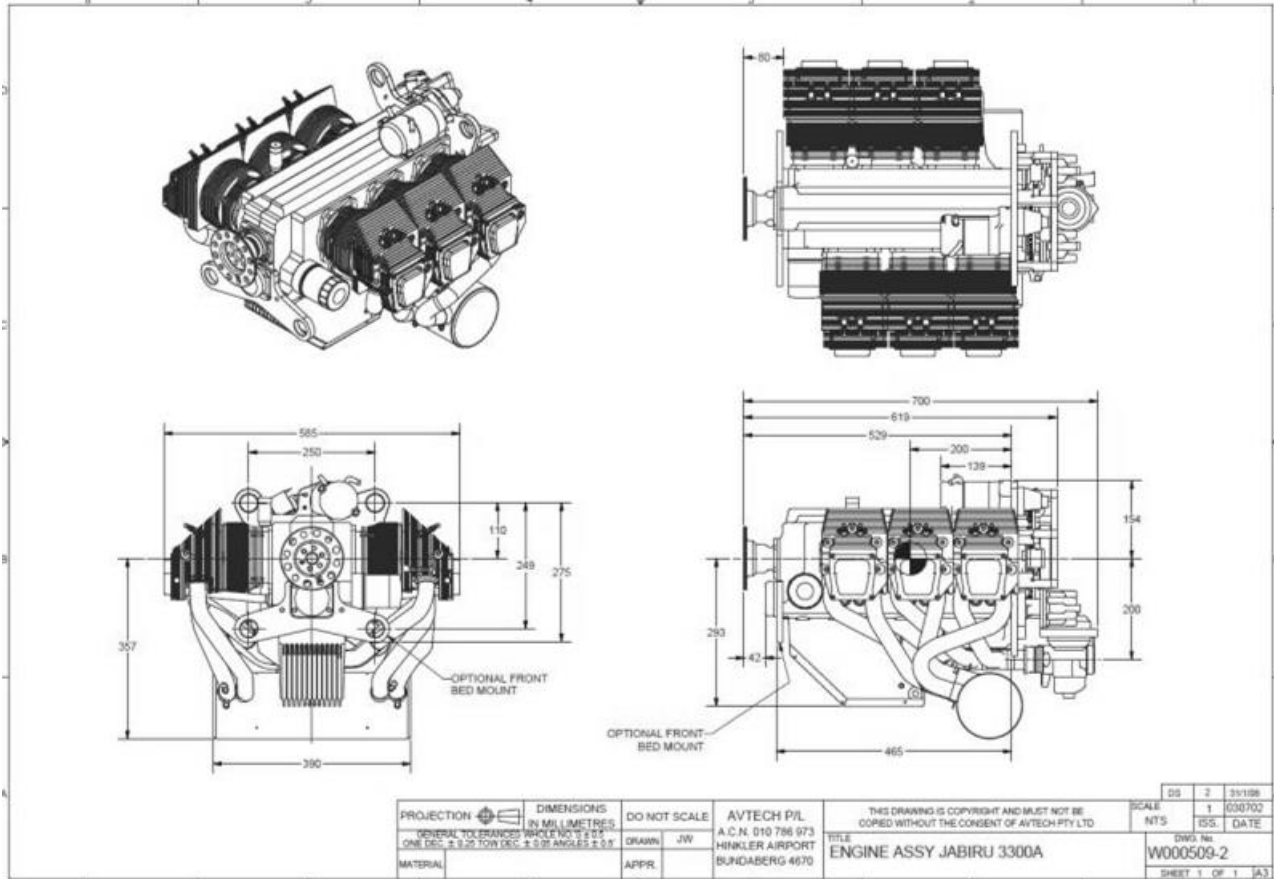
Figure 4 – 3300 Engine Dimensions
