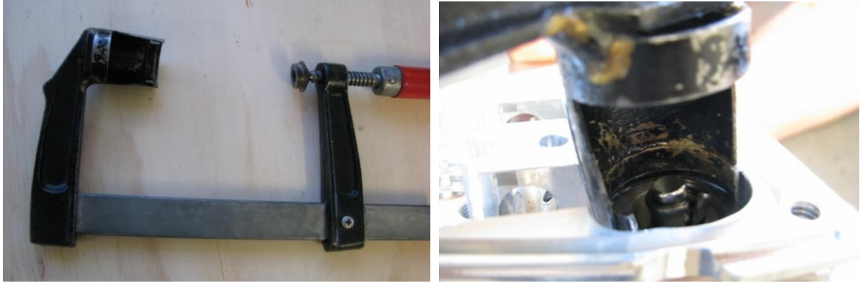
Figure 19 – Valve Spring Compressor / Collet Remover
