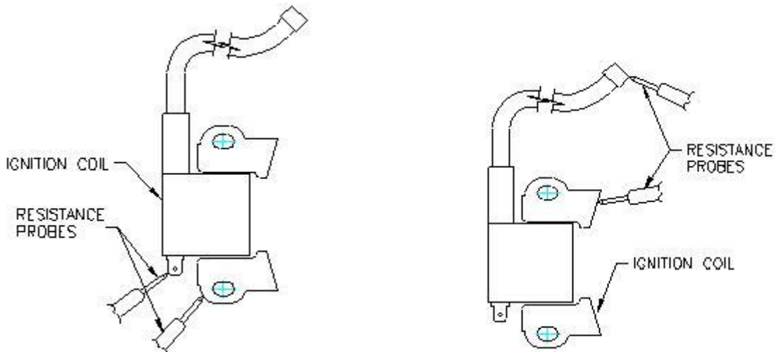
Drawing 9439064/1 IGNITION PRIMARY RESISTANCE Drawing 9439064/1 IGNITION SECONDARY RESISTANCE Figure 43 – Ignition Coil Tests
