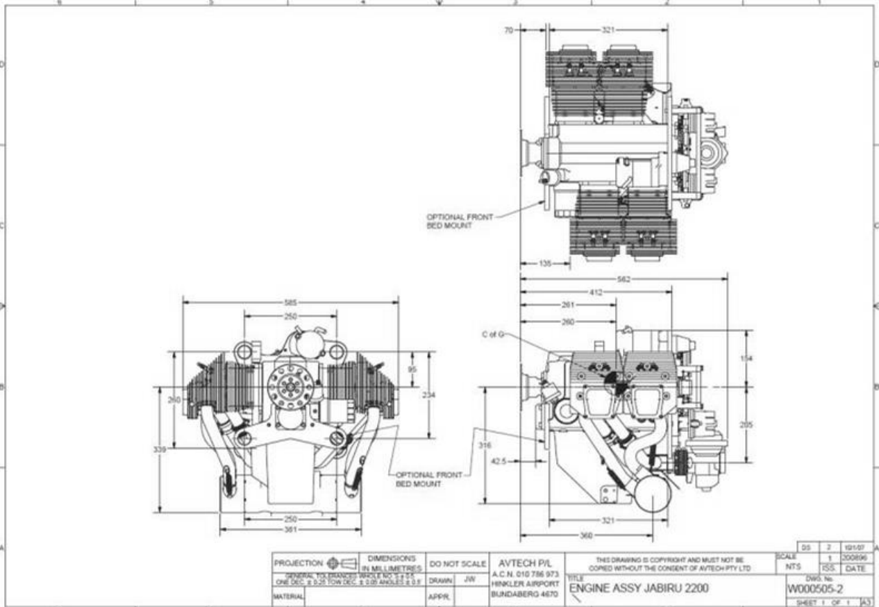
Figure 2 – 2200 Engine Dimensions
