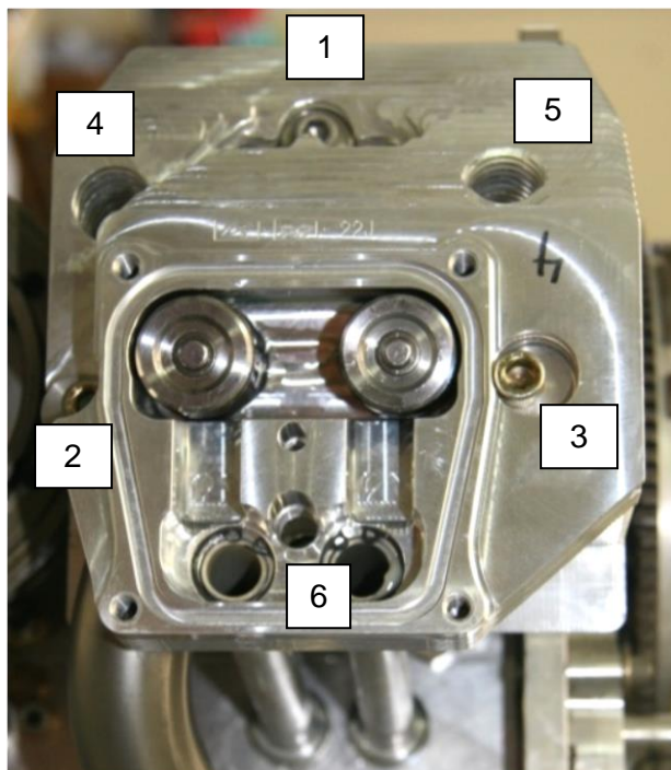
Figure 39 – Head Bolt Locations
