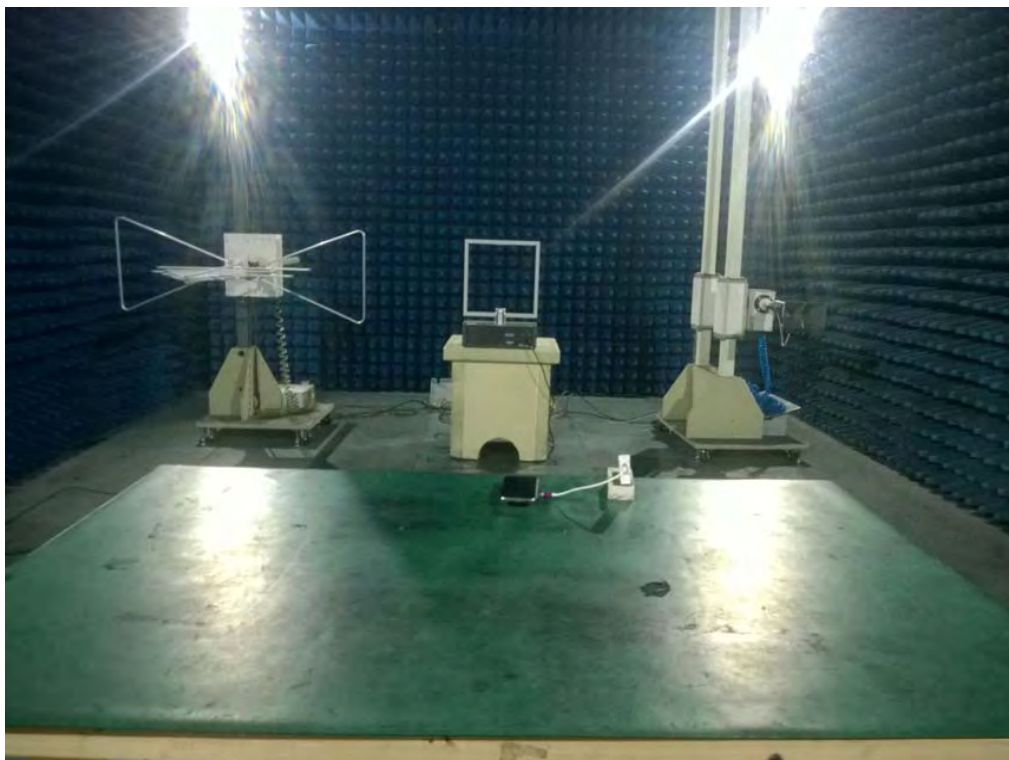
2 Photo of Radiation Emission Test
