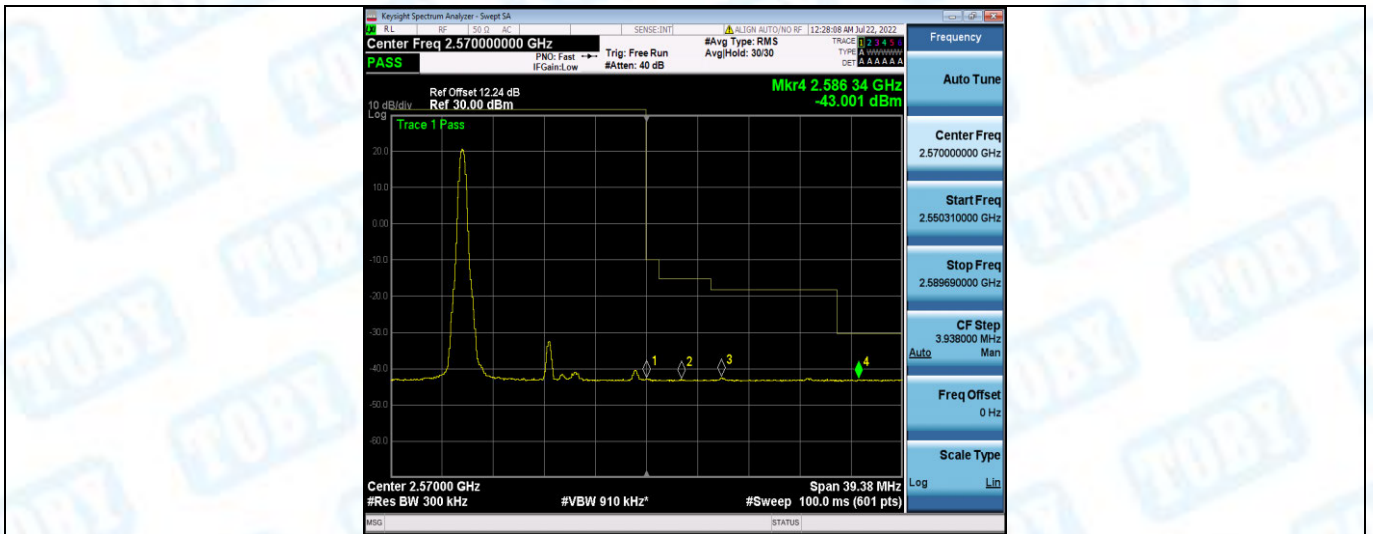
Band7-15MHz-16QAM-21375-1RB#74
