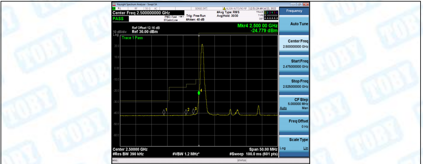
Band7-20MHz-QPSK-20850-1RB#99
