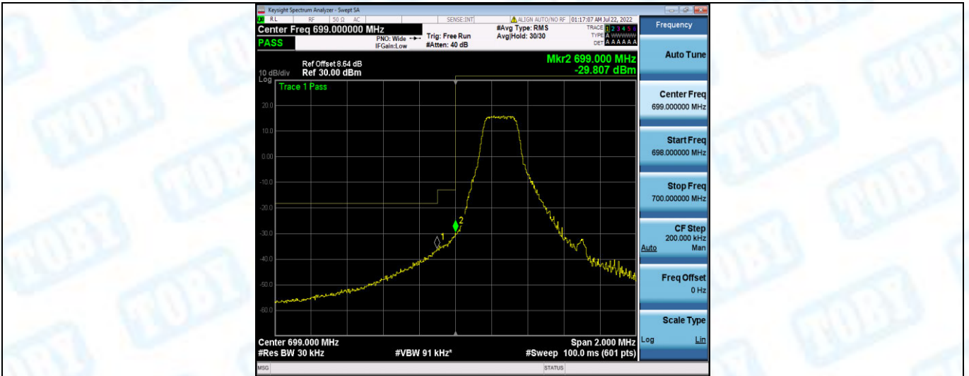
Band12-1.4MHz-16QAM-23017-1RB#5
