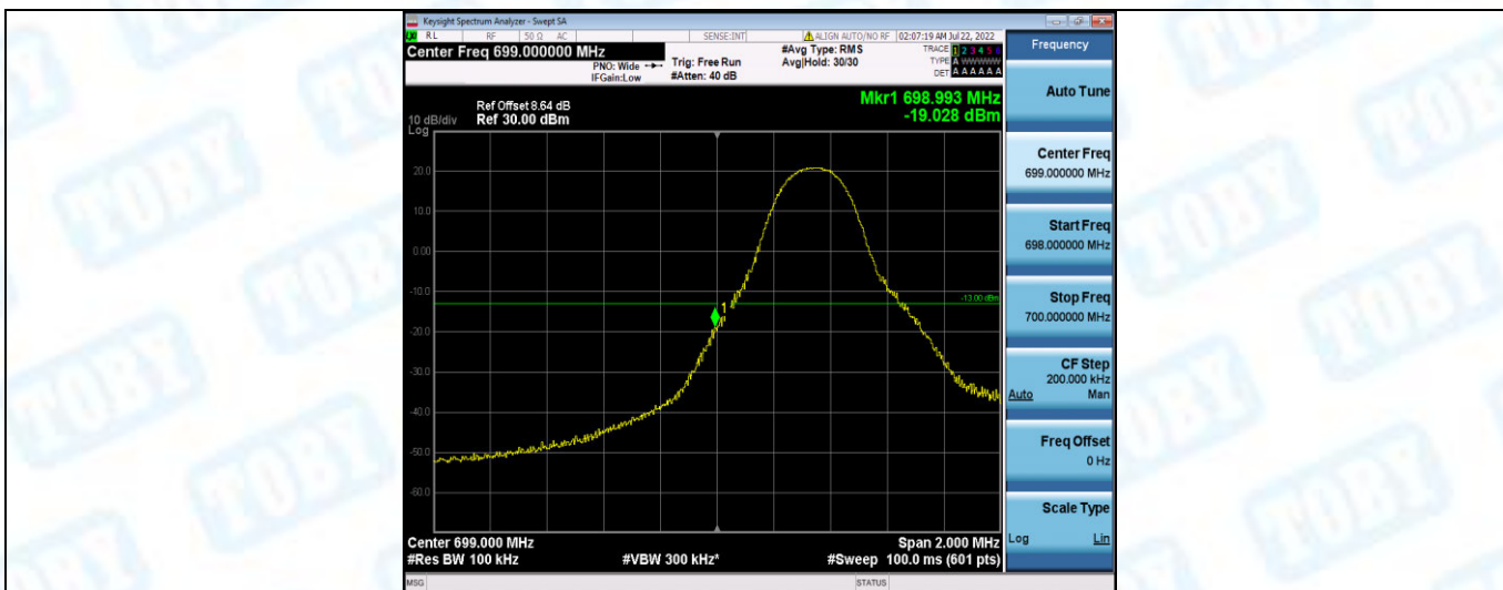
Band12-5MHz-16QAM-23035-1RB#24
