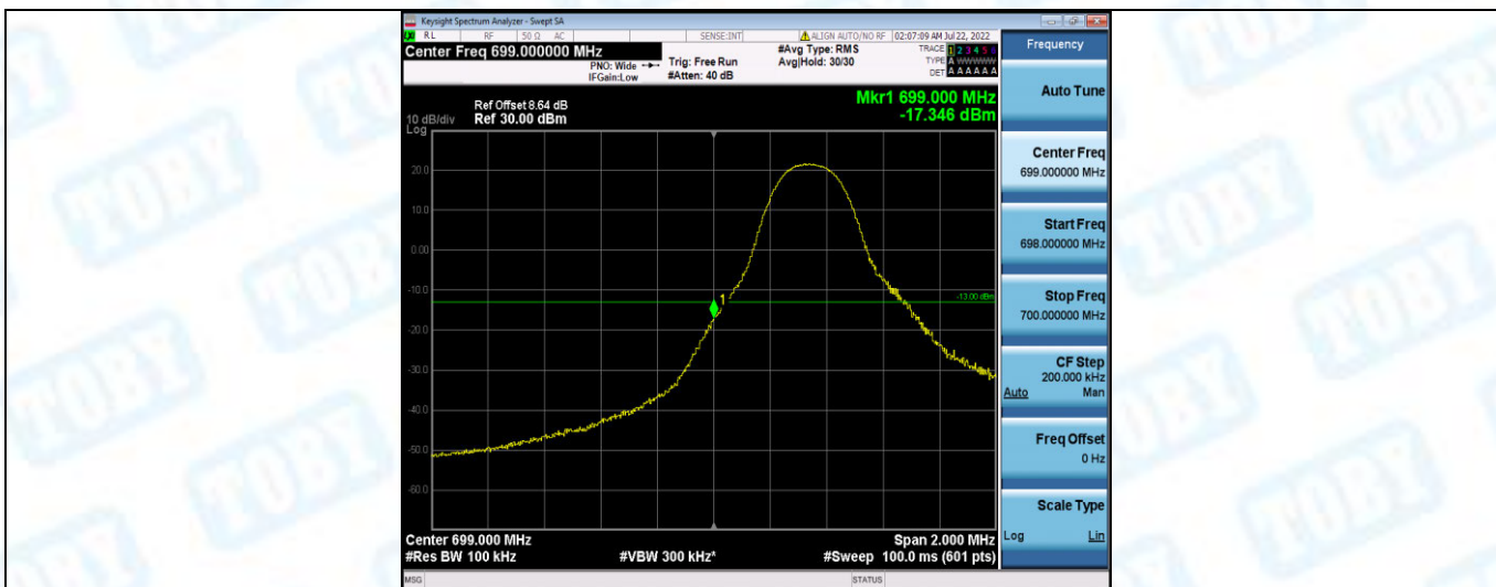
Band12-5MHz-QPSK-23035-1RB#24
