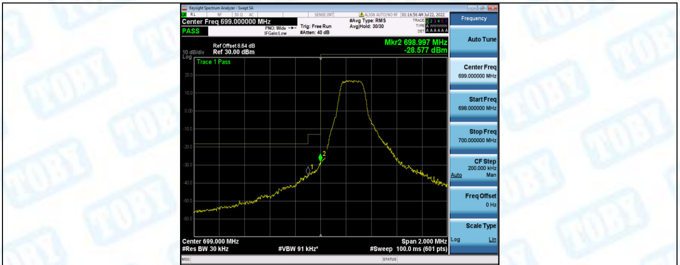
Band12-1.4MHz-QPSK-23017-1RB#5
