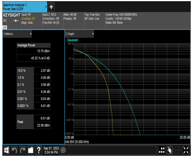
Band5-5MHz-16QAM-20525-1RB#0
