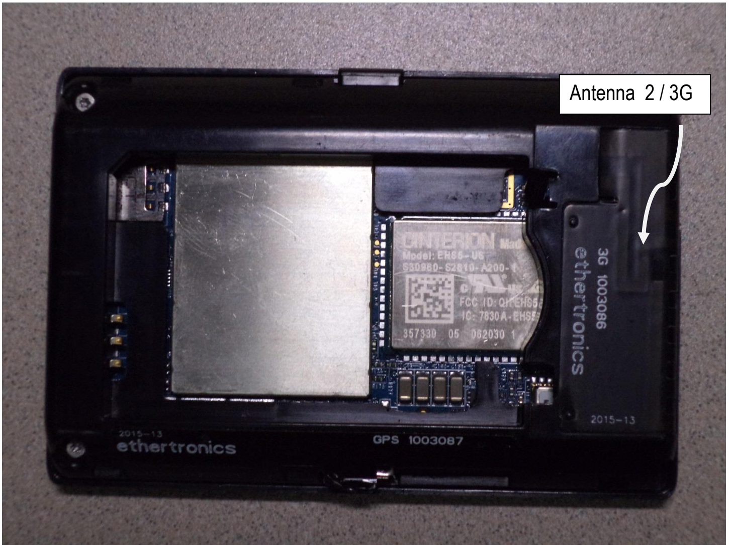
Photo 1: Antenna Locations
