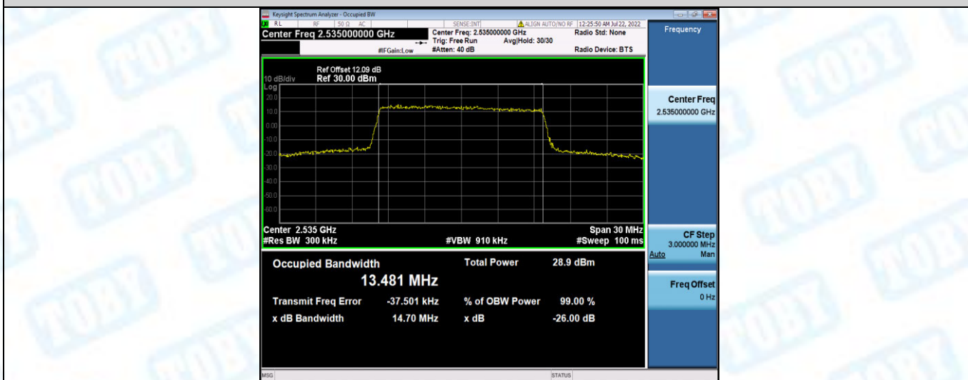
Band7-15MHz-16QAM-21375-75RB#0
