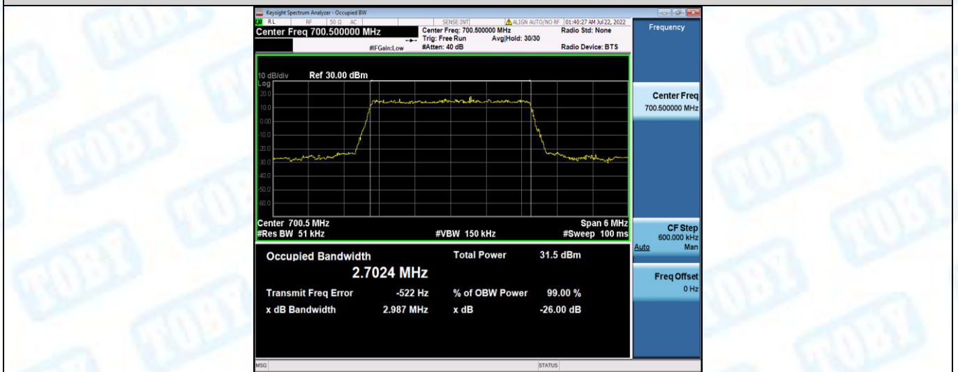
Band12-3MHz-QPSK-23095-15RB#0
