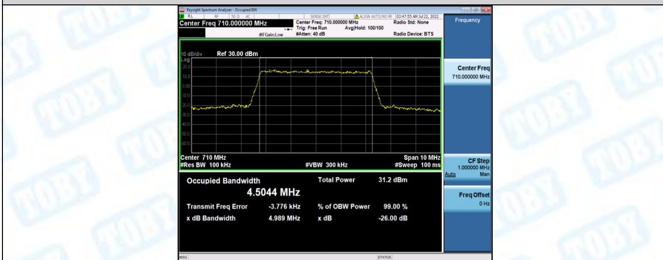
Band17-5MHz-QPSK-23825-25RB#0
