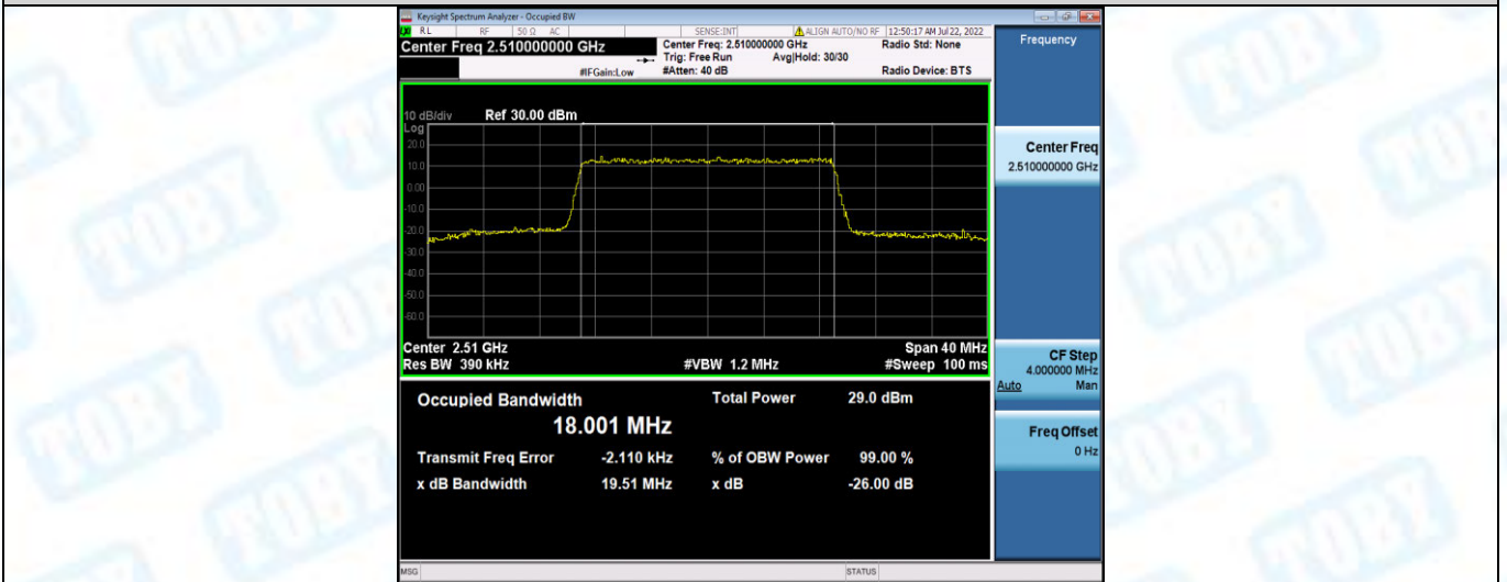
Band7-20MHz-16QAM-21100-100RB#0
