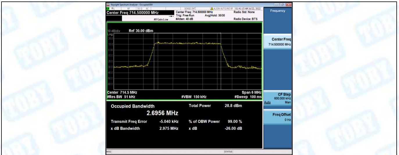
Band12-5MHz-QPSK-23035-25RB#0
