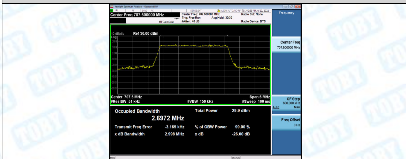
Band12-3MHz-16QAM-23165-15RB#0
