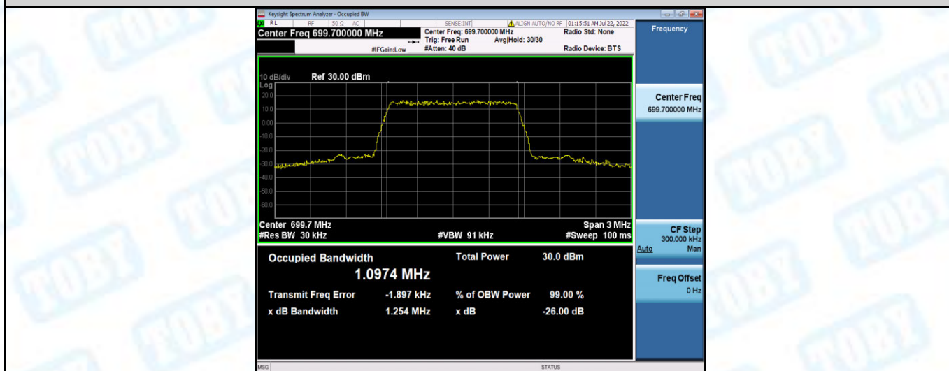
Band12-1.4MHz-16QAM-23095-6RB#0
