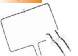
W10779716 (3600W/240V) Whirlpool Range bake element. 20.50"W x 16.75"L x 3.5" insert
