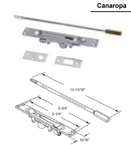
11-1801 Nickel Single Flush Bolt with rod, 12", tip and keeper for Steel/Wood Doors
