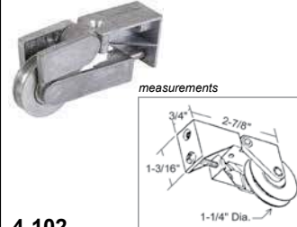
4-102 Sliding Glass Door Roller, 3/4" Wide, Single Mounting Hole
