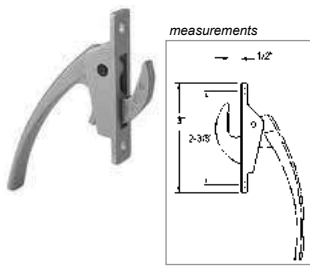
6-1345 Brown 6-1345SL Silver Window casement & awning. Locking Handle. die cast
