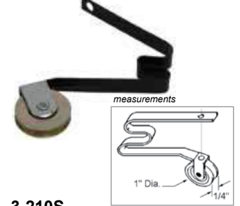
3-210S 1" O.D. Steel Ball Bearing
