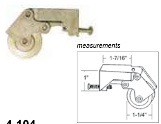
4-104 1 1/4" Die Cast Housing Steel B.B. Wheel
