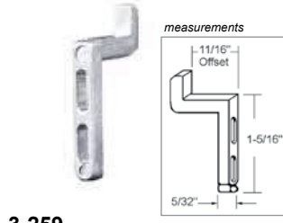
3-259 Sliding Screen Door Strike (11/16" Offset)
