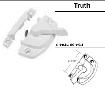
6-1363W White Truth Entrygard Die Cast Cam Lock. c/w lugs. OEM 17.19.32.200, 171932200
