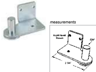
11-1502L Left Hand 11-1502R Right Hand Commercial Door Pivot - Bottom Frame Portion Right Hand Shown.
