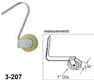
3-207 Steel Ball Bearing Wheel, 1/4" wheel width x 1" dia.
