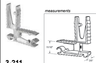
3-211 Sliding Screen Door Corner. Used with 3-202 sliding screen door roller. Die cast
