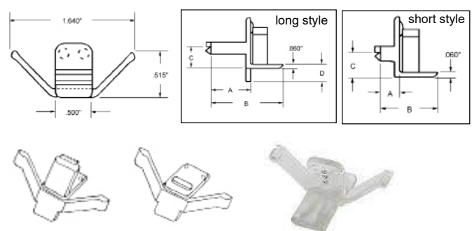
3-214 Bottom Sliding Screen Corner Bracket
