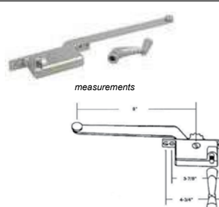
7-1368L Left 7-1368R Right Casement Operator Right Hand Shown.
