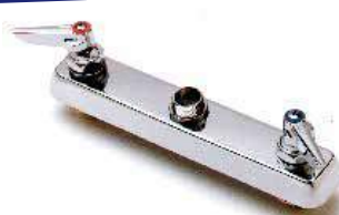
B-1120-LN 8" Deck mounted, Bronze body, removable seats, 10-1/2" long X 2" wide chrome plated escutcheon, 8" centers, 1-1/2" long shanks, 1/2" IPS thread
