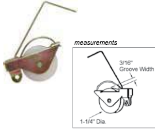
3-213 1 1/4" O.D. Nylon Wheel, 3/16" groove
