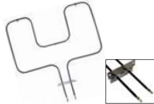
UB639 (3000W/240V) G.E. Range bake element. 18.50"W x 15.0"L x 4.0" insert
