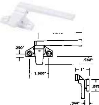
6-1332LB Left/Brown 6-1332RB Right/Brown 6-1332LW Left/White 6-1332RW Right/White Cam Handle Offset Base, Right Hand Shown, use with 6-1332 strike, other colours avail.
