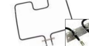
UB593 (3000W/240V) Universal Range bake element. 17.50"W x 15.05"L x 1.875" insert
