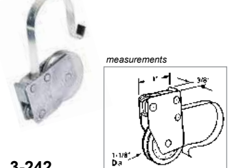
3-242 Sliding Screen Door Roller. Used with 3-287 corner. Steel wheel
