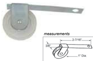
3-306 Sliding Screen Door Roller, plastic wheel, 1" dia.
