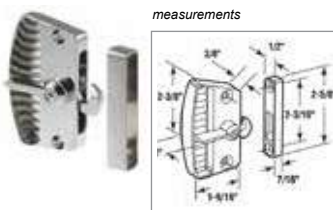
PL-A105 Sliding Screen Door Deluxe Latch & Pull, 2-3/8", Diecast, Chrome, Non-Handed
