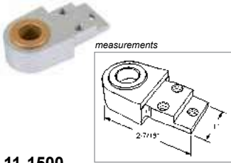
11-1500 Zimmcor Aluminium Top Frame Portion
