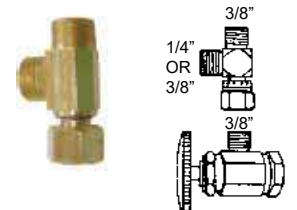
ULN299A 3/8" X 3/8" ULN299 3/8" X 1/4" EZ-Connect Adapters, Makes Water appliance hook-up easy. Use when installing an icemaker, dishwasher.
