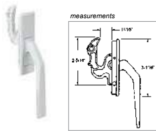
6-1335 White Window casement & awning. Locking Handle. Mounting holes: 2-1/2"
