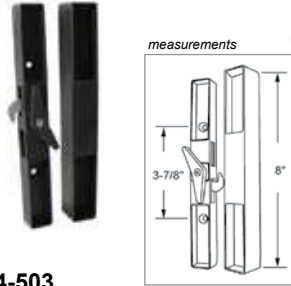
4-503 Black Plastic Handle 8"H, 3-7/8" centers
