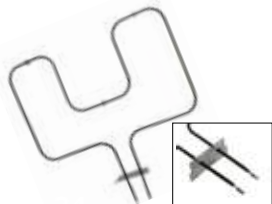
WG02F05396 (3000W/240V) G.E. Range bake element. 18.0"W x 16.0"L x 4.0" insert
