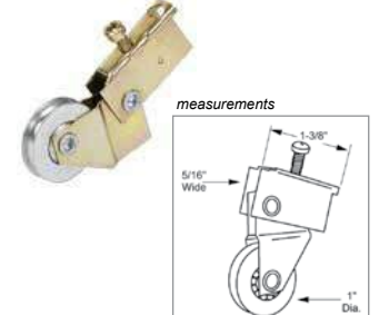
3-233 Sliding Screen Door Roller, steel w/ball bearing
