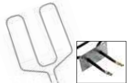
WS01F02162 (2565/3410W) G.E. Range Broil Element 14.5"W x 16.5"L x 2.6" insert
