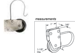
3-240 1 1/8" Dia. Plastic Wheel Use with #3-287 Corner
