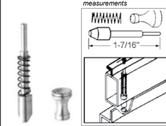
3-258 Sliding Screen Door Strike (9/32" Offset)
