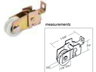
4-133 Nylon B.B. Wheel Steel Housing 1-5/8"H x 7/8"D roller
