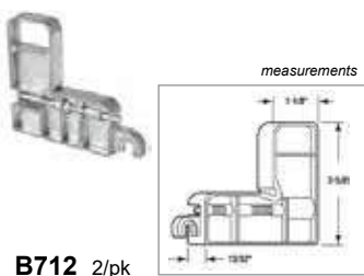
B712 2/pk Sliding Screen Door Corner. Narrow style corner - die cast
