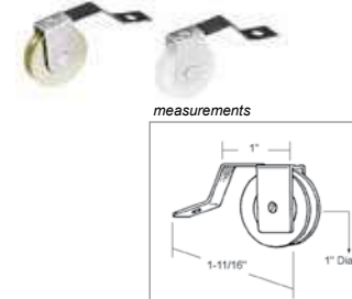
3-241 nylon roller 3-241S steel ball bearing Sliding Screen Door Roller
