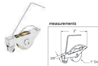
B541 St. ball bearing 2/pk 3-303-N Nylon each Sliding Screen Door Rollers, 1" Dia.
