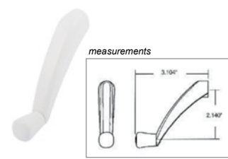
6-1467W White 6-1467B Brown Window casement & awning. Window Crank Handle (Contour) (Truth Hardware 5/16" Spline 11454)
