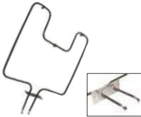
318255006 (3000W/240V) Frigidaire Range replacement bake element. 20"W x 15.5"L x 4.00" insert.
