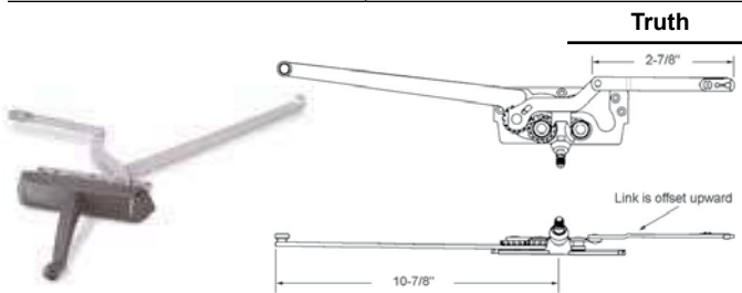
Right 6-1374R A = 3-13/16" Left 6-1374L Left A = 3-13/16" 6-1343R A = 4-7/16" Left 6-1343L Left A = 4-7/16" Truth entry guard operators, dual arm, cover not included (6-1355). Use with 6-1354 Track. Use 6-1301 Series handles
