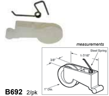
B692 2/pk Plastic Wheel & Housing
