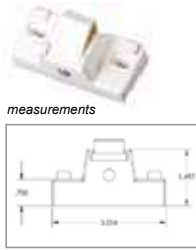
101-305WH Foot activated sliding door lock. Secondary security lock. 3" Length
