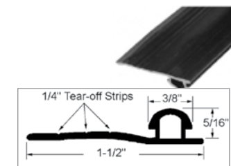
3-1459 Sliding Screen Door Bug Bar. Sold per foot. 5/16"W x 1-1/2"H
