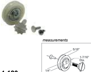
4-123 1 7/16" O.D. Nylon B.B. Wheel Off-Center Hole
