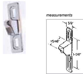
4-554A Die Cast Shim Door Strike 5/8"W, 1-5/8" centers, 15/16" projection
