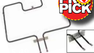
UB642 (3000W/240V) G.E./Camco Range bake element. 18.50"W x 14.55"L x 3.875" insert (WB44M147, RB147)
