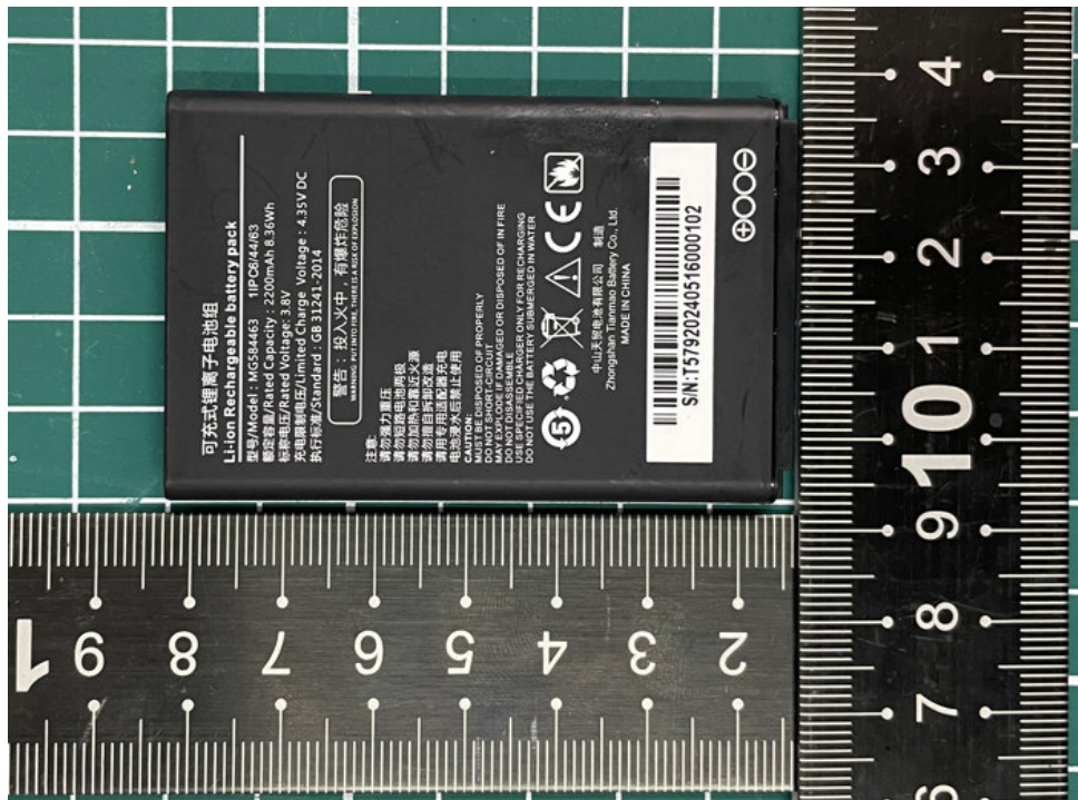
Battery 2
