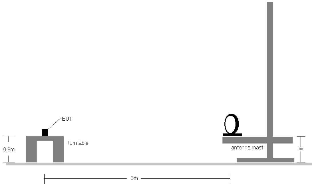
Figure 7-4. Radiated Test Setup
