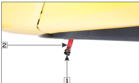
(1) Drain tube plug (2) Canister drain tube
