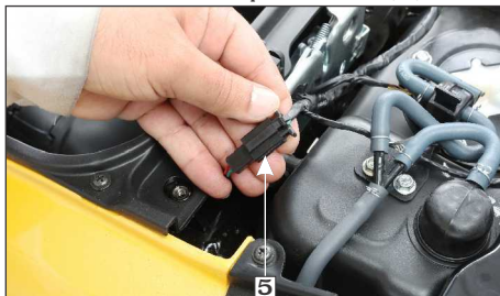
(5) Boot lamp connector
