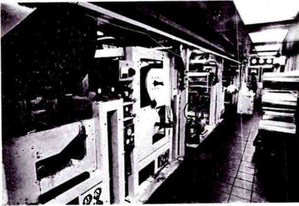
Above is but a small part of one of the giant coating machines: in this section the film is fed into the machine, coated, and exposed to a magnetic field to orient the iron-oxide particles.
