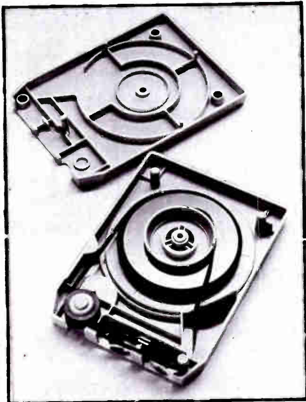
Inside view of the 8-track cartridge with its single reel and continuous loop of recording tape.
