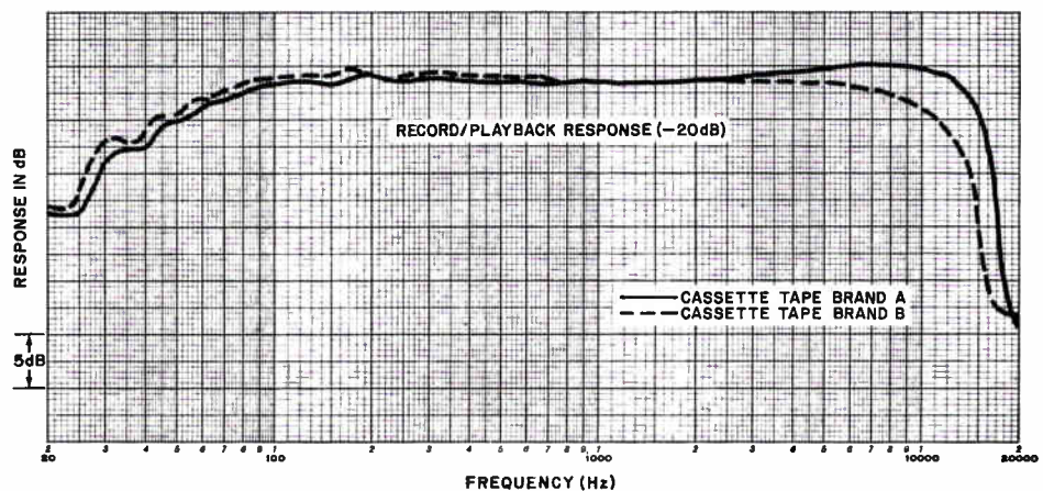
Difference in over-all frequency response with change of tape formulation (at fixed "Std" bias setting).
