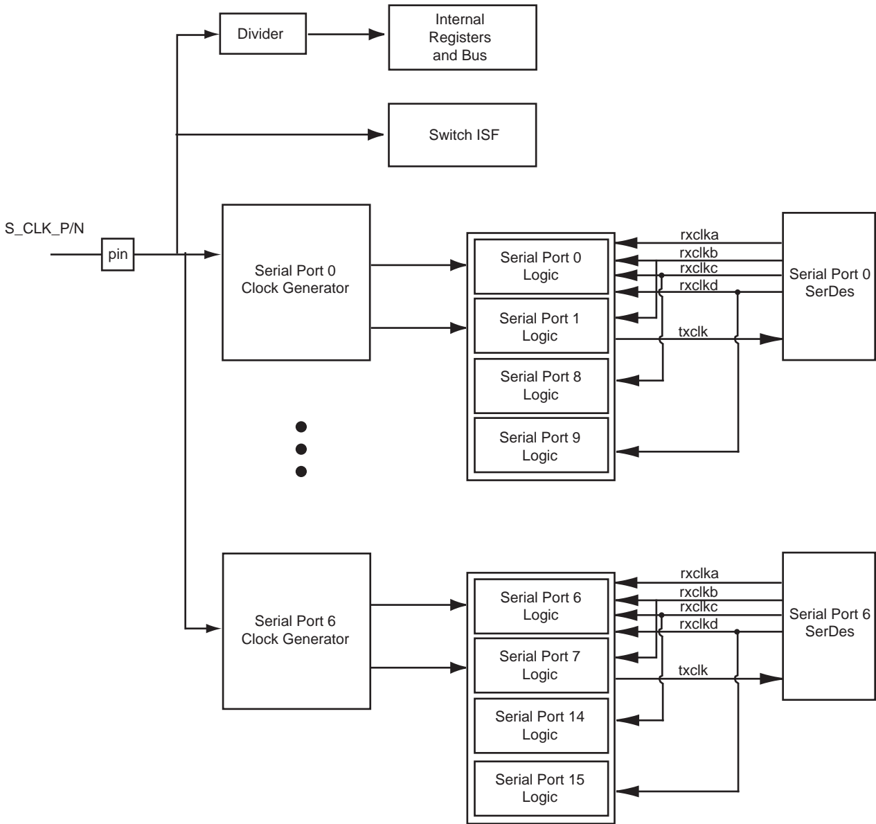
Figure 47: Clock Architecture
