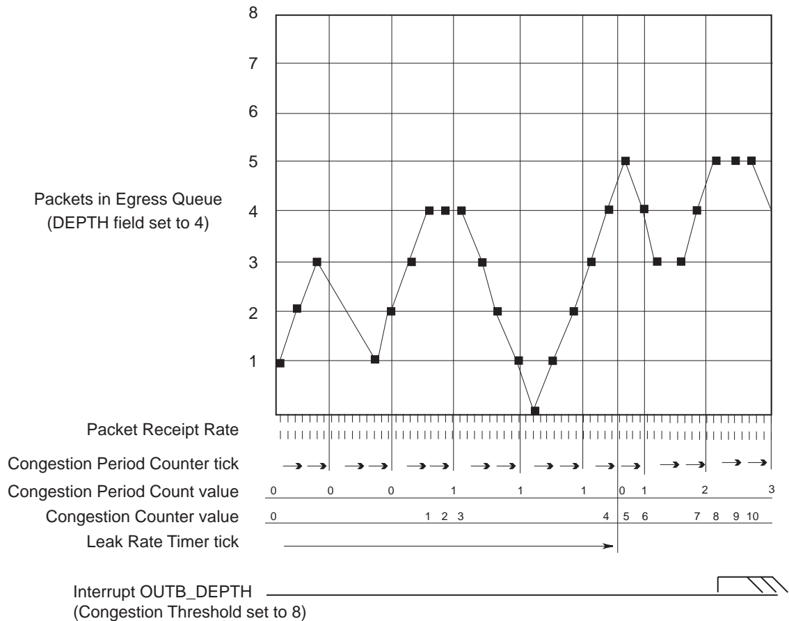
Figure 44: Congestion Example
