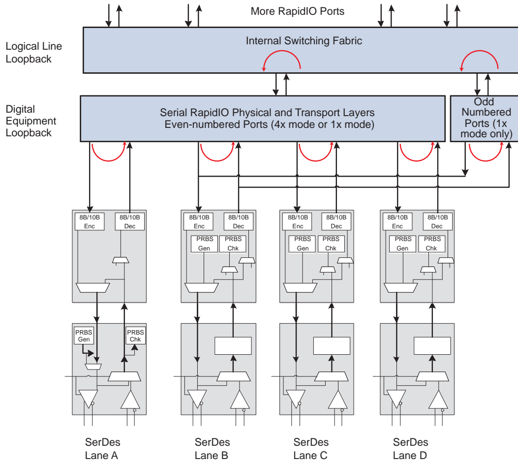
Figure 15: Tsi577 Loopbacks
