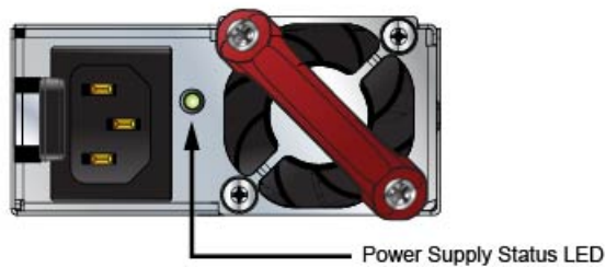
Figure A-5: AC Power Supply Status LED
