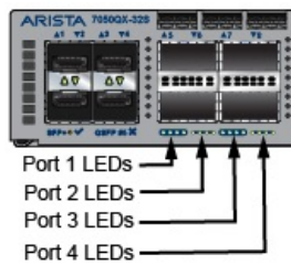
Figure A-3: Port LEDs
