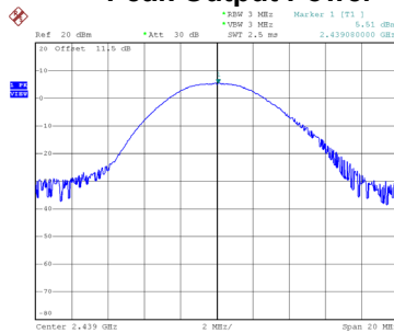
CH13 Peak Output Power
