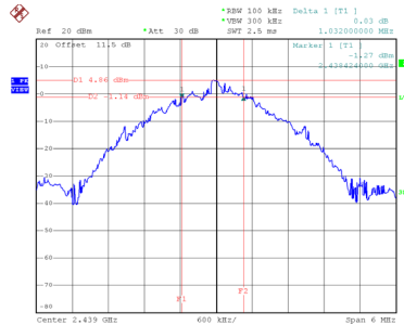
CH13 6 dB Bandwidth
