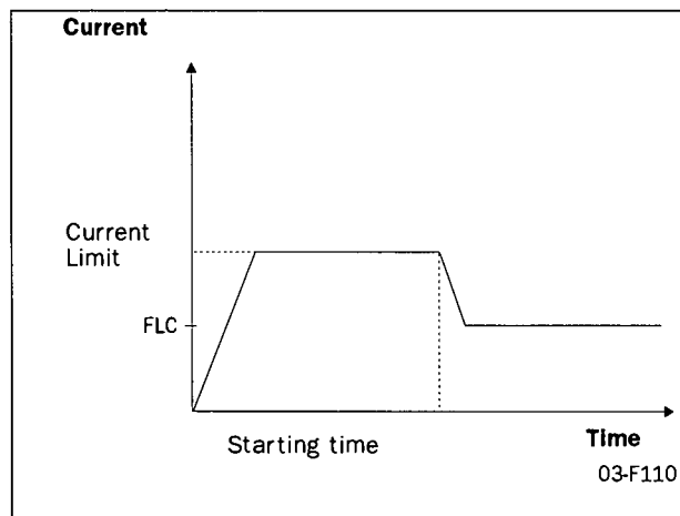
Fig. 35 Current limit
