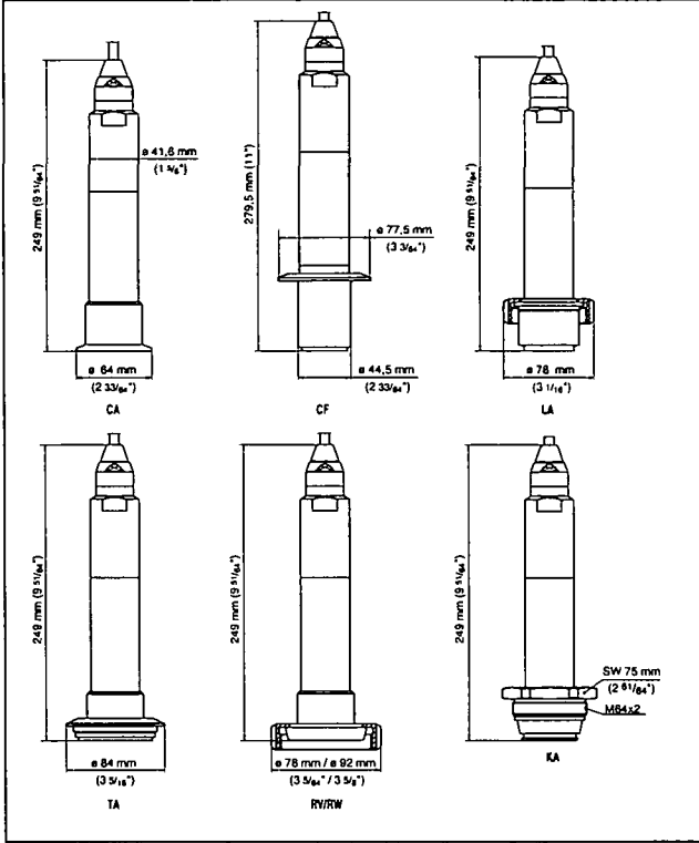
Fig. 18: VEGABAR 75 - hygienic fitting: CA/CF = Tri-Clamp 2"/Tri-Clamp 2 1/2", LA = hygienic fitting with compression nut F40, TA = Tuchenhagen Varivent DN 32, RV/RW = bolting DN 40/DN 50 according to DIN 11851, KA = conus DN 40, AA = DRD
