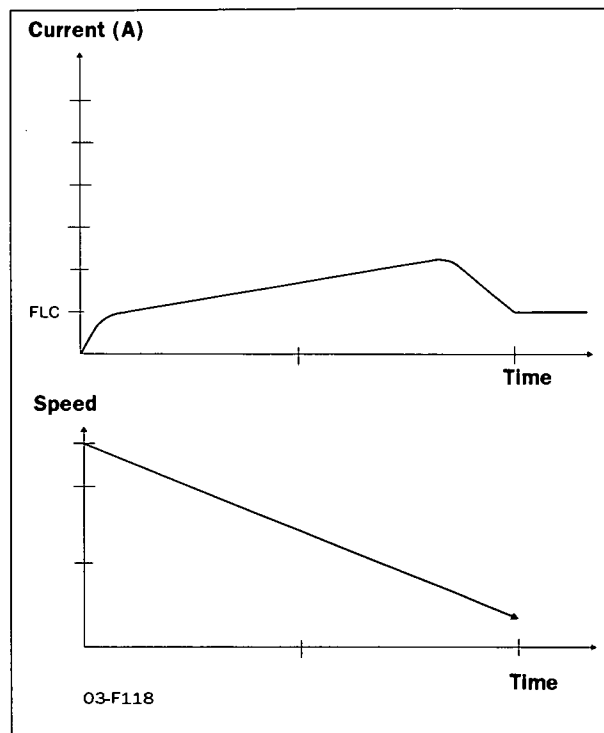
Fig. 36 Pump control
