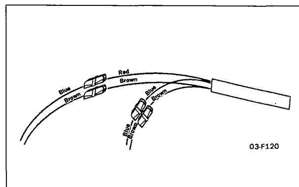
Fig. 63 Cable kit
