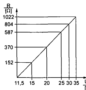
Temperature head transmitter load chart for estimating the load resistance. Additional resistances have to be subtracted from the value calculated as shown in the equation.
