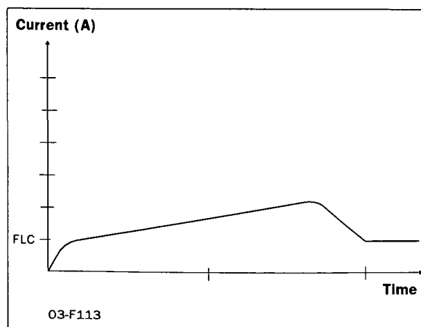
Fig. 5 Torque control
