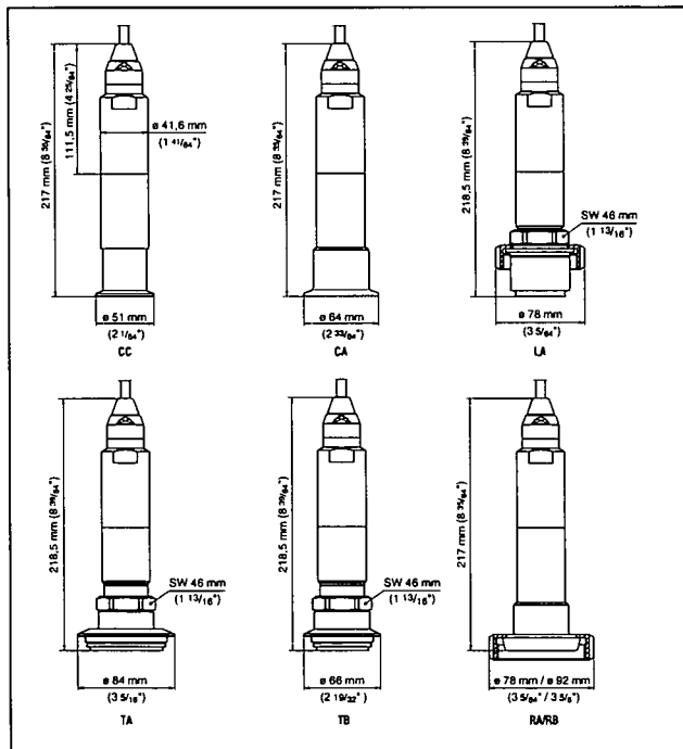
Fig. 12: VEGABAR 74 - hygienic fitting: CC = Tri-Clamp ½", CA = Tri-Clamp 2", LA = hygienic fitting with compression nut F40, TA = Tuchenhagen Varivent DN 32, TB =
