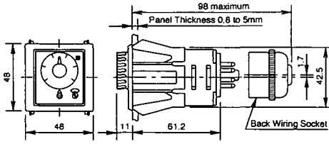
Analog GT3 Timer, 8-Pin and 11-Pin with SR6P-S08 or SR6P-S11
