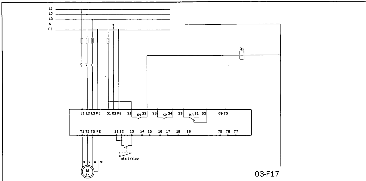
Fig. 6 Standard wiring.
